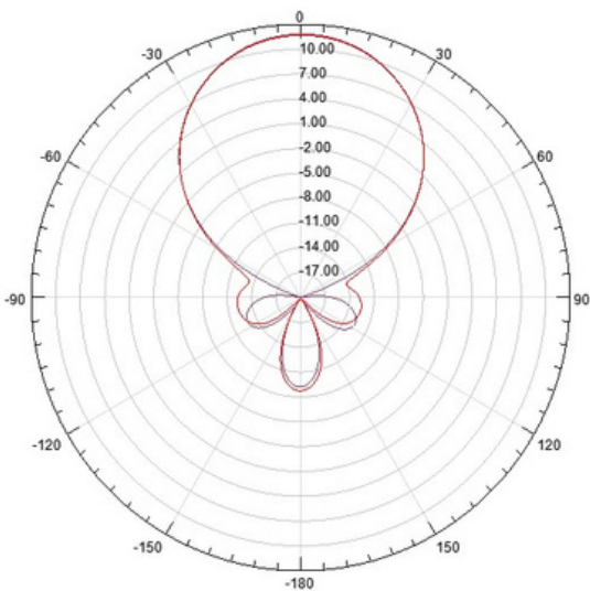
Radiation Pattern M Plane 757-788MHz 3dB Beamwidth 48°
