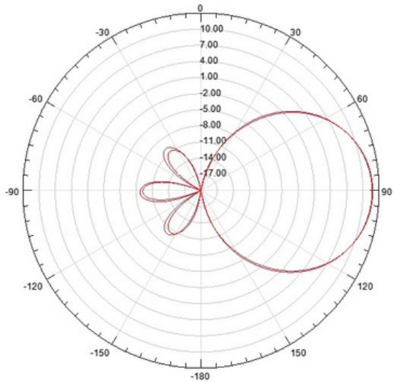
Radiation Pattern E Plane 757-788MHz 3dB Beamwidth 46°
